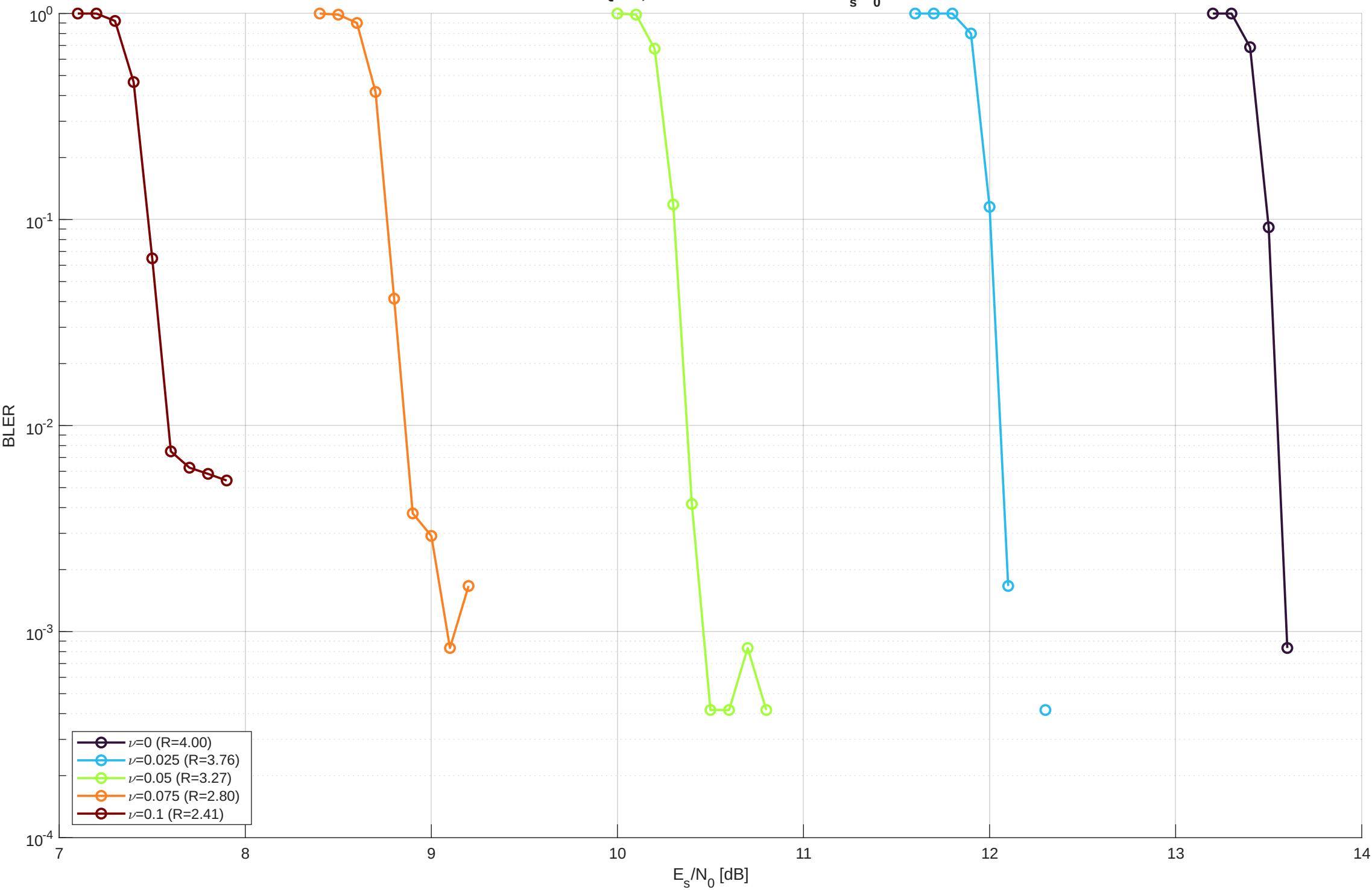
PAS 64-QAM, DVB-S2 2/3 — BLER vs E_s/N_0
